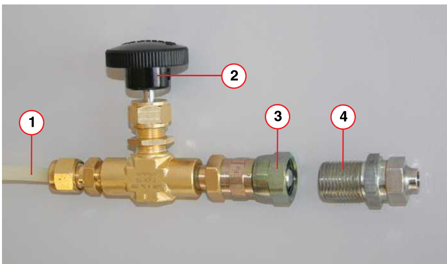
Fig. 380: He compressor - charge and vent adaptor (gas charging tool)
