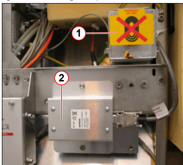
Fig. 350: Service Magnet Stop button
