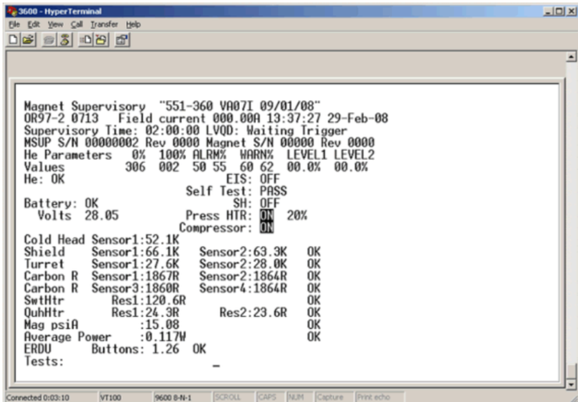
Fig. 377: MSUP 2657B - Process Display screen (typical)
