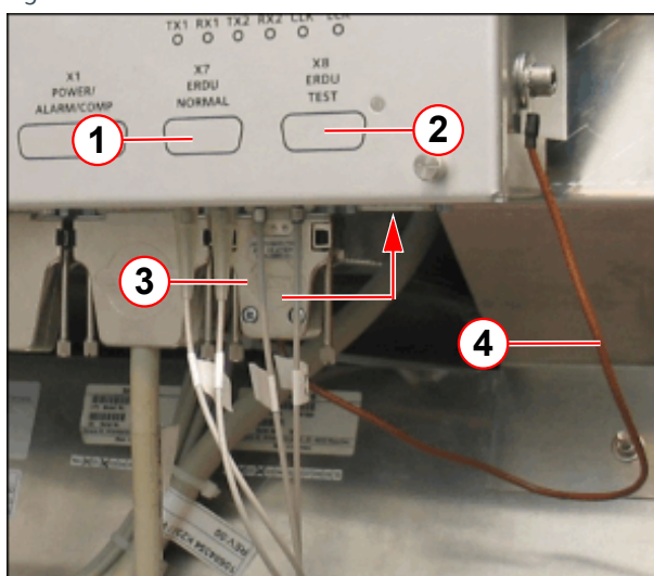
Fig. 351: ERDU test connector
