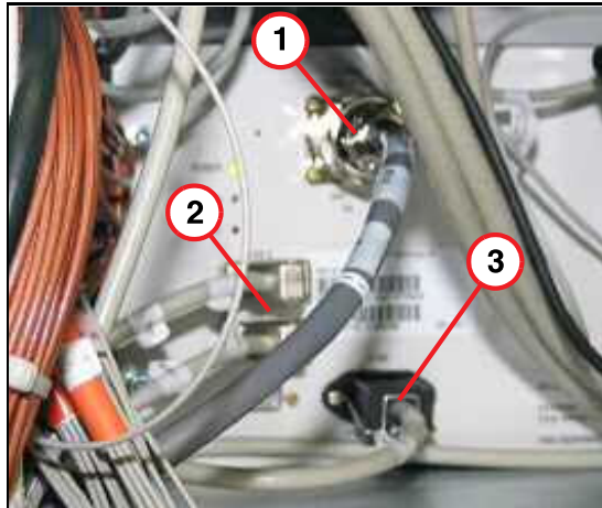
Fig. 365: Shim power supply
