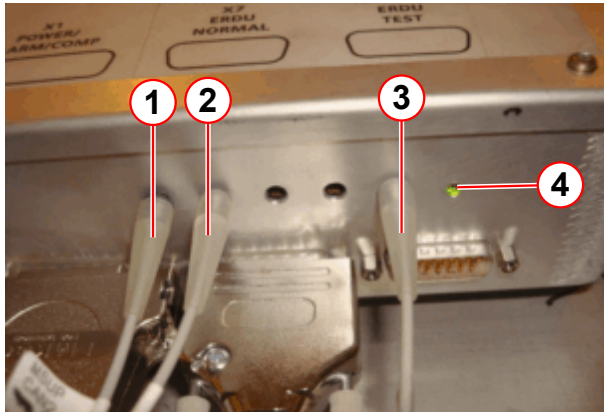
Fig. 315: MSUP 2306 fiber optic cables
