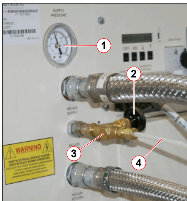
Fig. 386: F70 - Charge & vent adaptor (gas charging tool)
