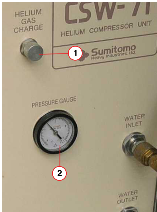
Fig. 379: Compressor He Gas charge & pressure gauge
