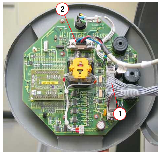
Fig. 346: Alarm box connectors
