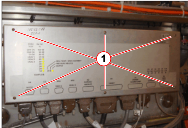
(1) M3 screws and washers (6 off)
