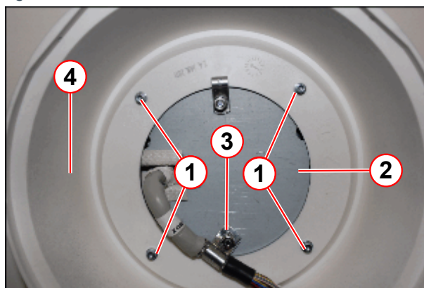
Fig. 355: Back of Alarm Box (inside)
