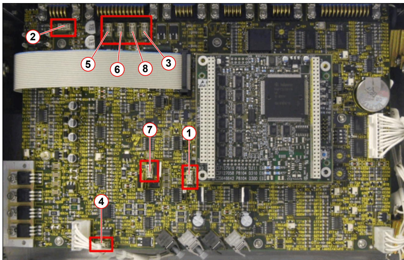
Fig. 374: MSUP 2657B - Fuses
