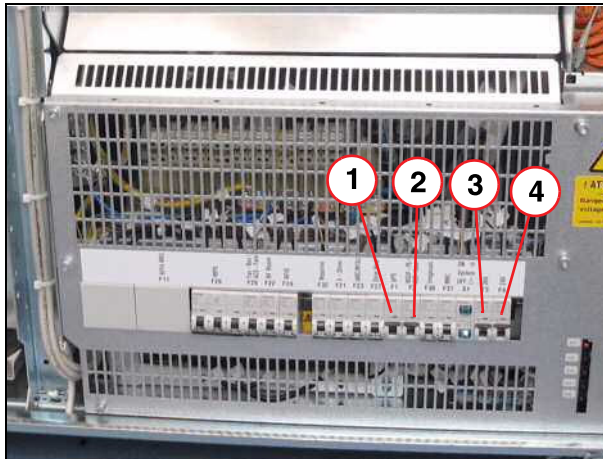
Fig. 352: ACC fuse (inside)
