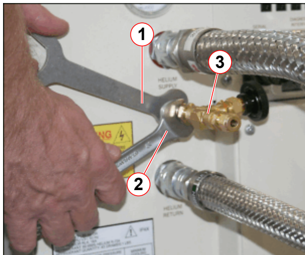
Fig. 385: F70 Compressor - Fit/remove charge & vent adaptor (gas charging tool)
