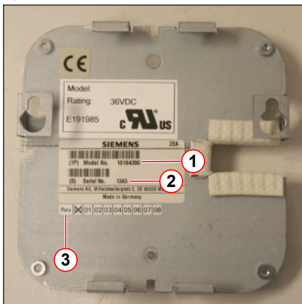
Fig. 348: Alarm box identification
