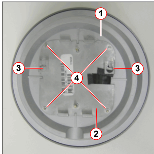
Fig. 357: Alarm box base - fixing plate
