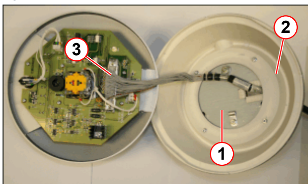
Fig. 354: Alarm box connector X1
