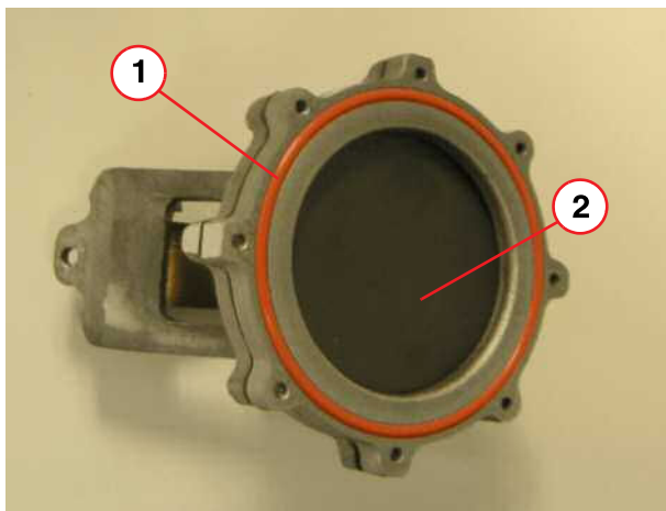
Fig. 12: Quench Valve Bursting Disk Assembly
