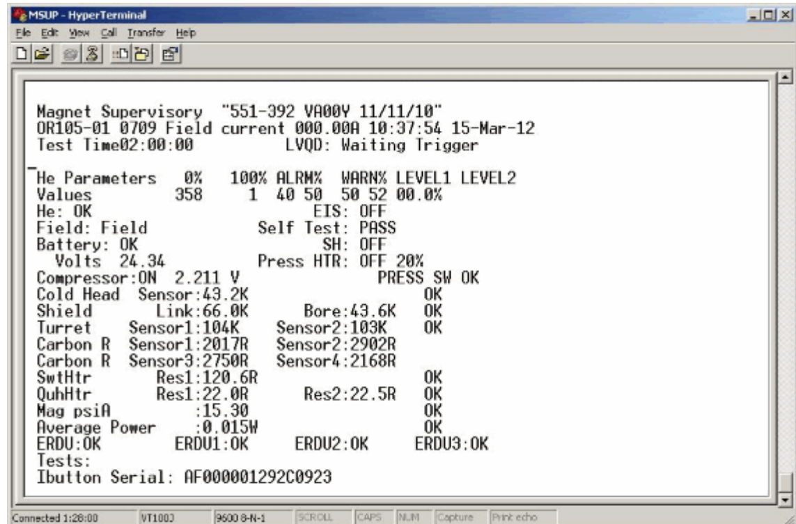
Fig. 367: MSUP Process display screen (Example)
