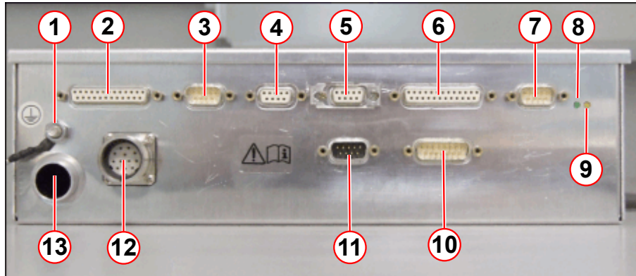
Fig. 376: MSUP 2657B - Indicators and input/output connections
