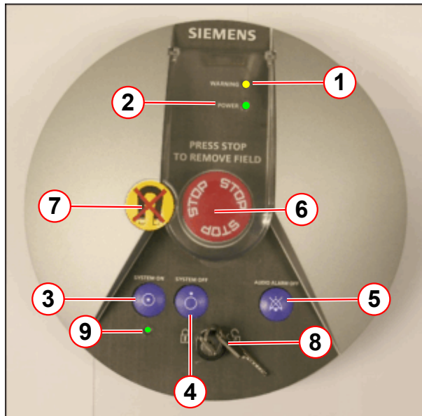
Fig. 359: Alarm box - LEDs and buttons
