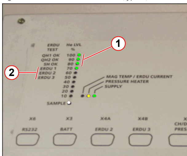
Fig. 360: ERDU test - LED indicators (typical)
