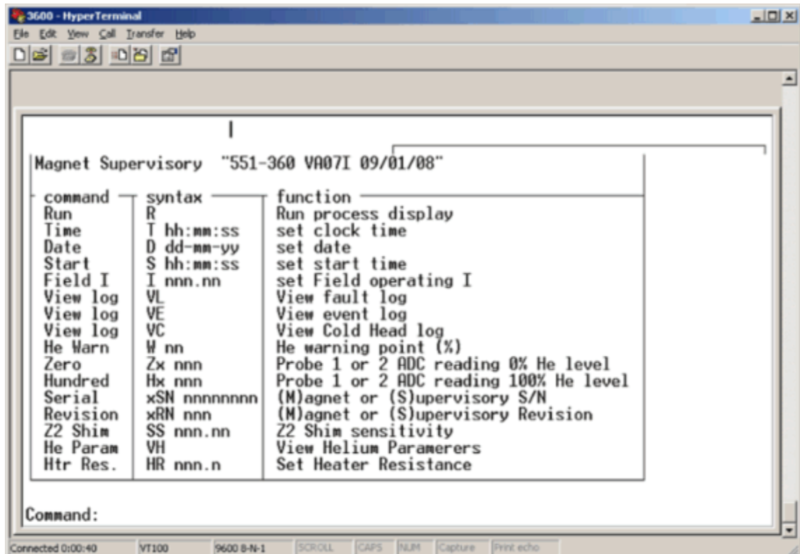
Fig. 378: MSUP 2657B - Command Input screen (typical)
