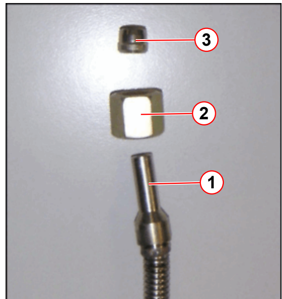
Fig. 73: WIKA Pressure switch compression joint
