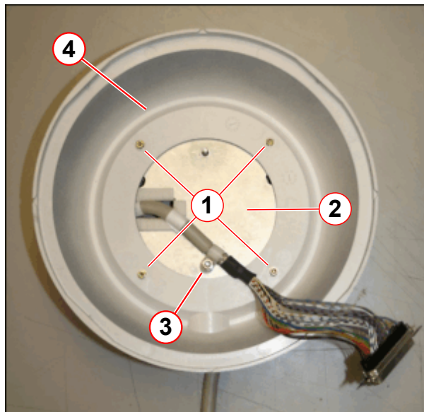
Fig. 347: Back of Alarm Box (inside)
