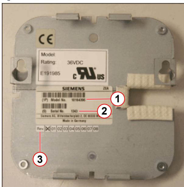
Fig. 358: Alarm box identification
