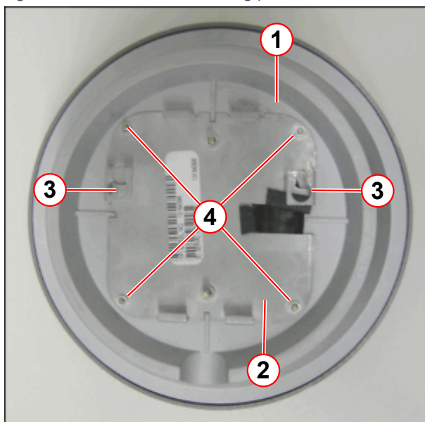
Fig. 349: Alarm box base - fixing plate
