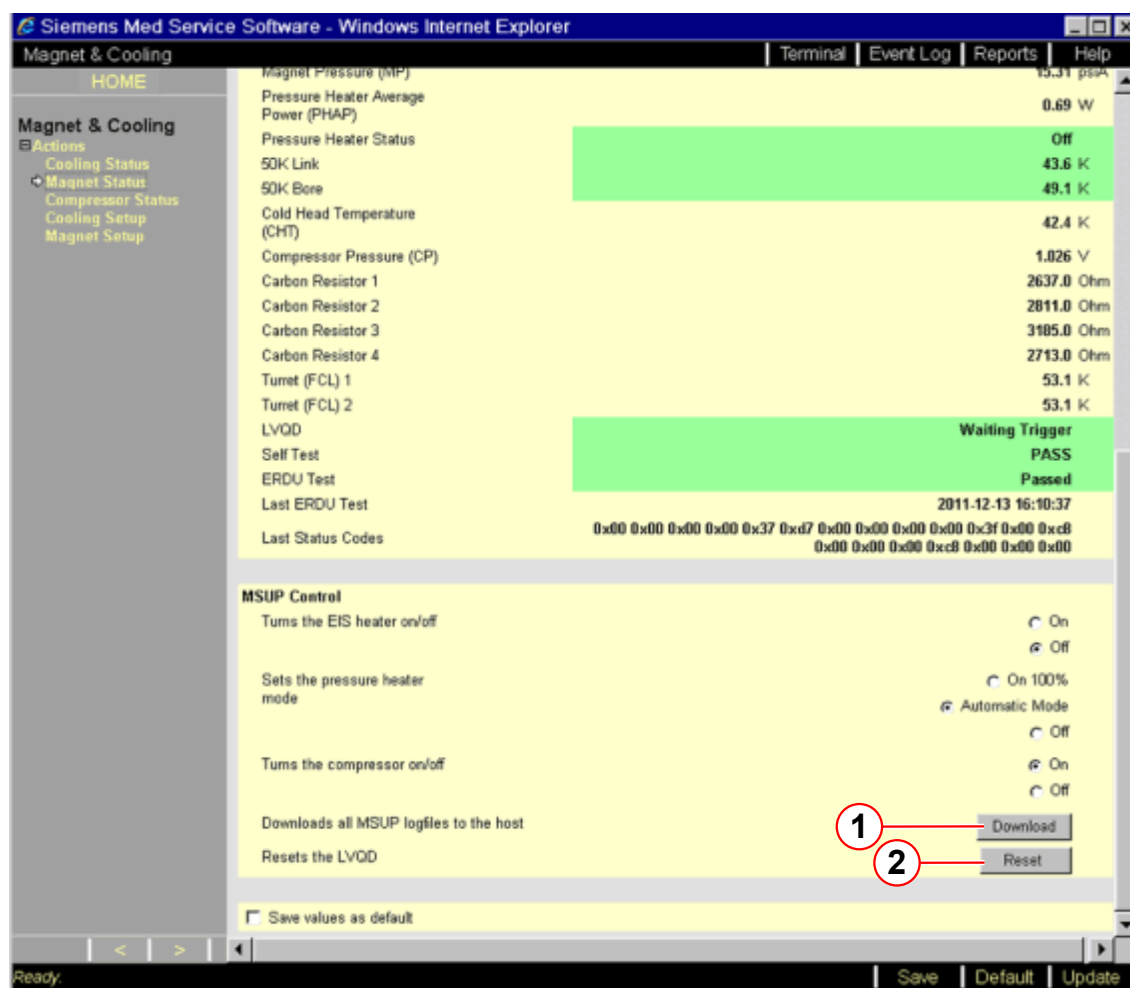
Fig. 368: Downloading MSUP logfiles to the Host
